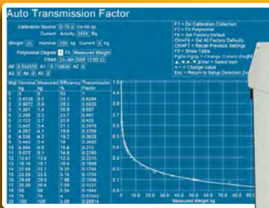
Auto Transmission Factor Calibration Screen
